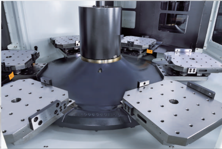
8 Pallets Unit
