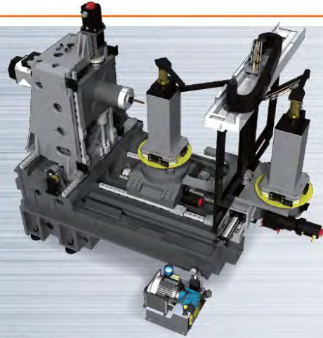
Hydraulic Overhead Arms for Fixtures
