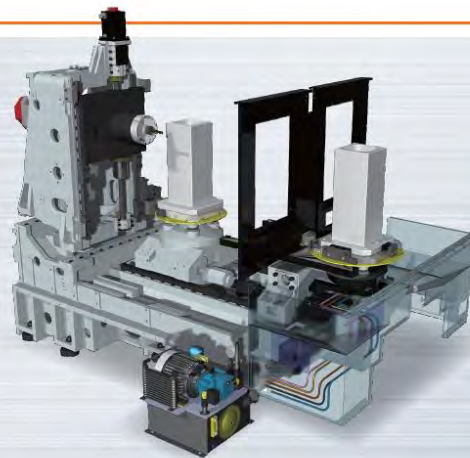
Hydraulic Thru Pallets for Fixtures
