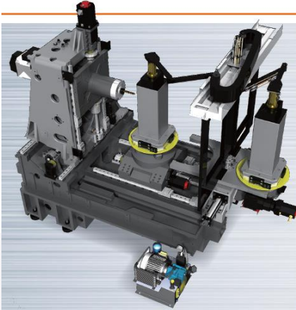
Hydraulic Overhead Arms for Fixtures
