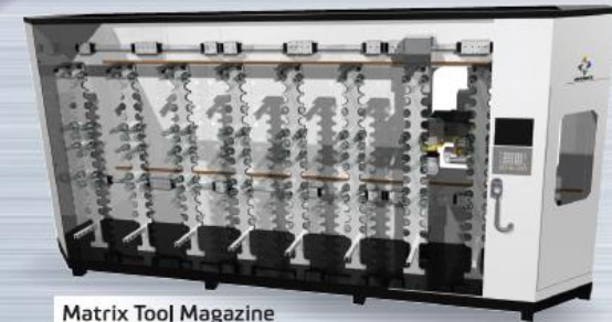
Matrix Tool Magazine
