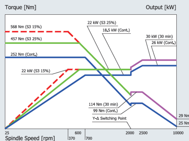
■ BBT 50 / 10,000 rpm Direct Drive Spindles [ST]
