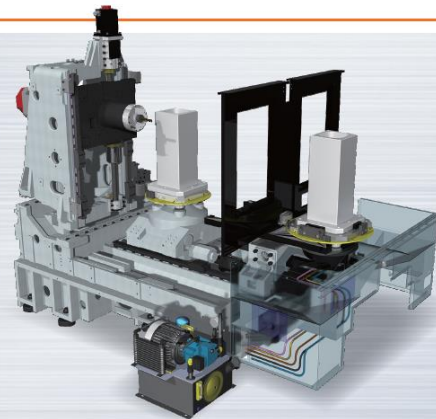
Hydraulic Thru Pallets for Fixtures
