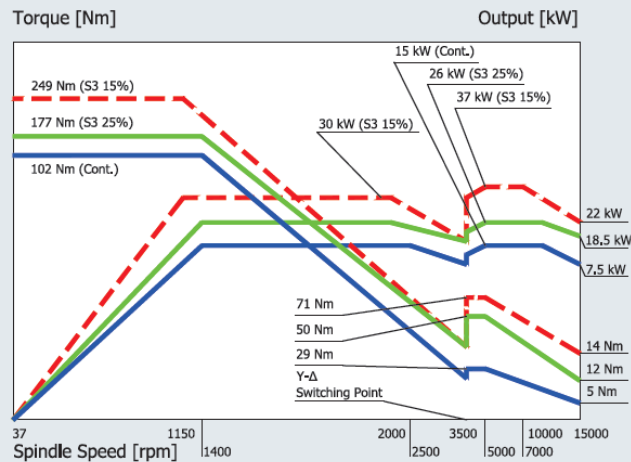
■ BBT 40 / 15,000 rpm Direct Drive Spindles [ST]
